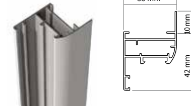
Z155 Telaio a Z "Z" shaped framework profile
