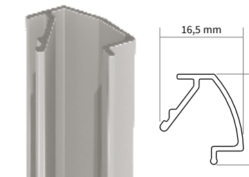
Z151 Copri filo anta Shutter cover profile
