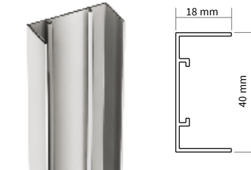
Z156 Compensatore telaio a L "L" shaped framework profile - balancer
