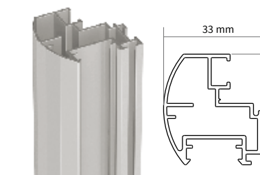
Z150 Profilo anta Shutter profile
