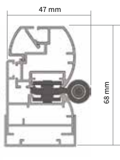
Telaio a L con compensatore anta e cerniera "L" shaped framework with balancer shutter and joint
