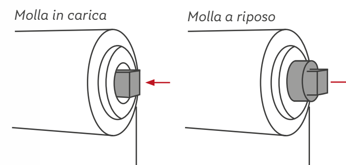
Rallentatore / Speed reducer
