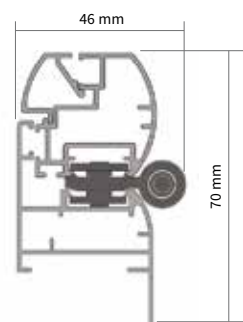
Telaio a Z con anta e cerniera "Z" shaped framework with shutter and joint
