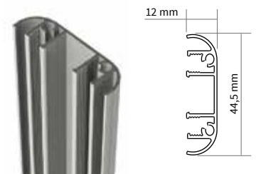
Z152 Traversa centrale Central crossbeam profile
