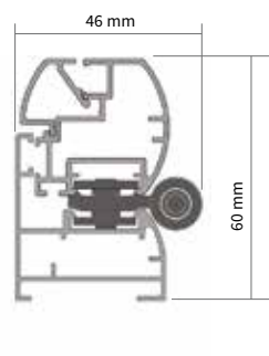
Telaio a L con anta e cerniera "L" shaped framework with shutter and joint
