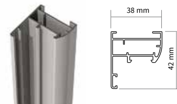
Z155 Telaio a L "L" shaped framework profile
