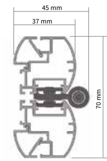
Profili anta + cerniera Shutter profile + joint
